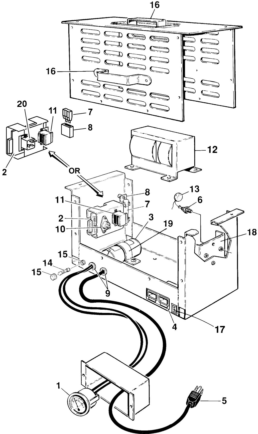
FIGURE 1-6.BATTERY CHARGER ASSEMBLY
