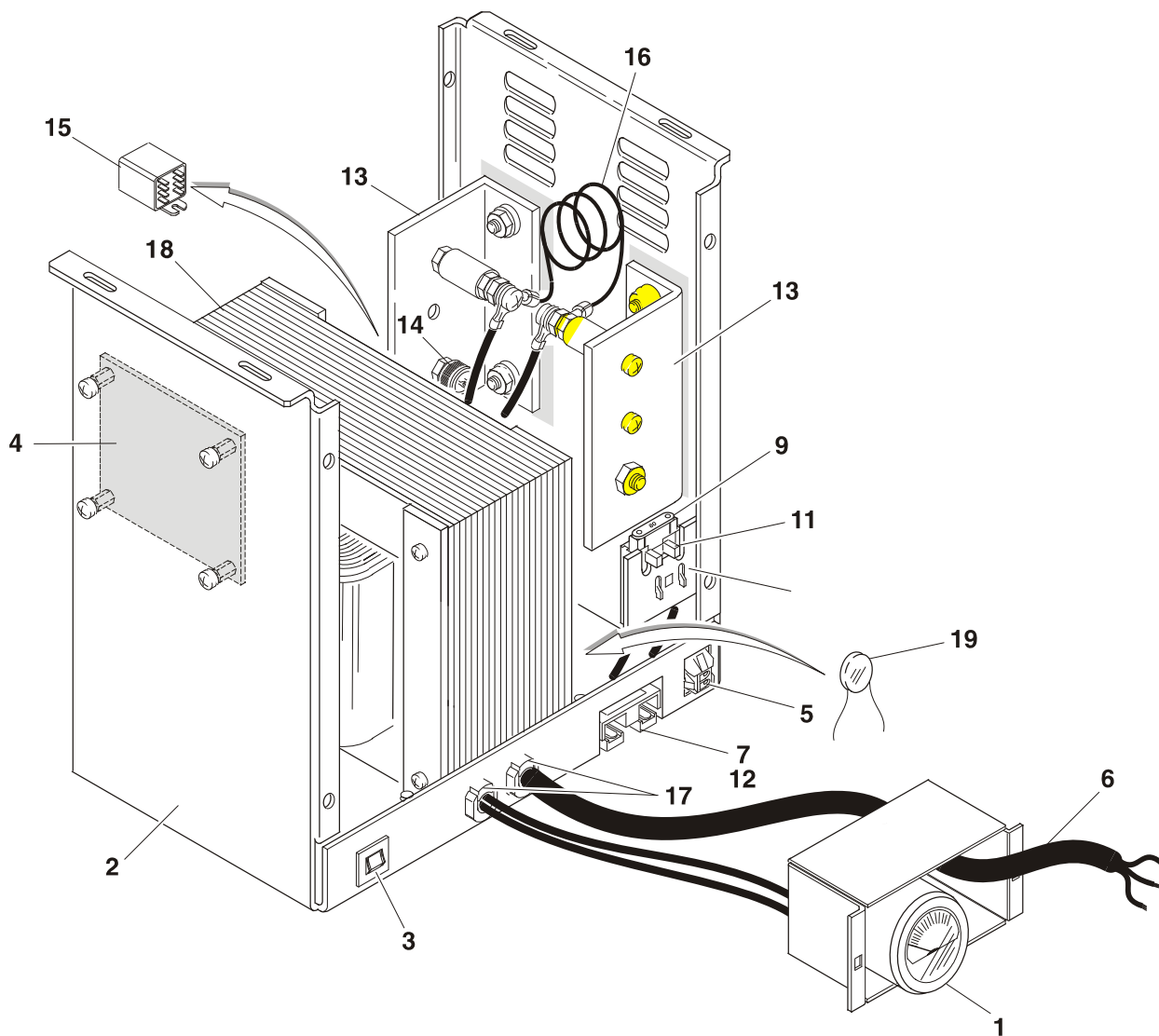
FIGURE 1-7.BATTERY CHARGER ASSEMBLY - 220VAC/50HZ (SERVICE REPLACEMENT)
