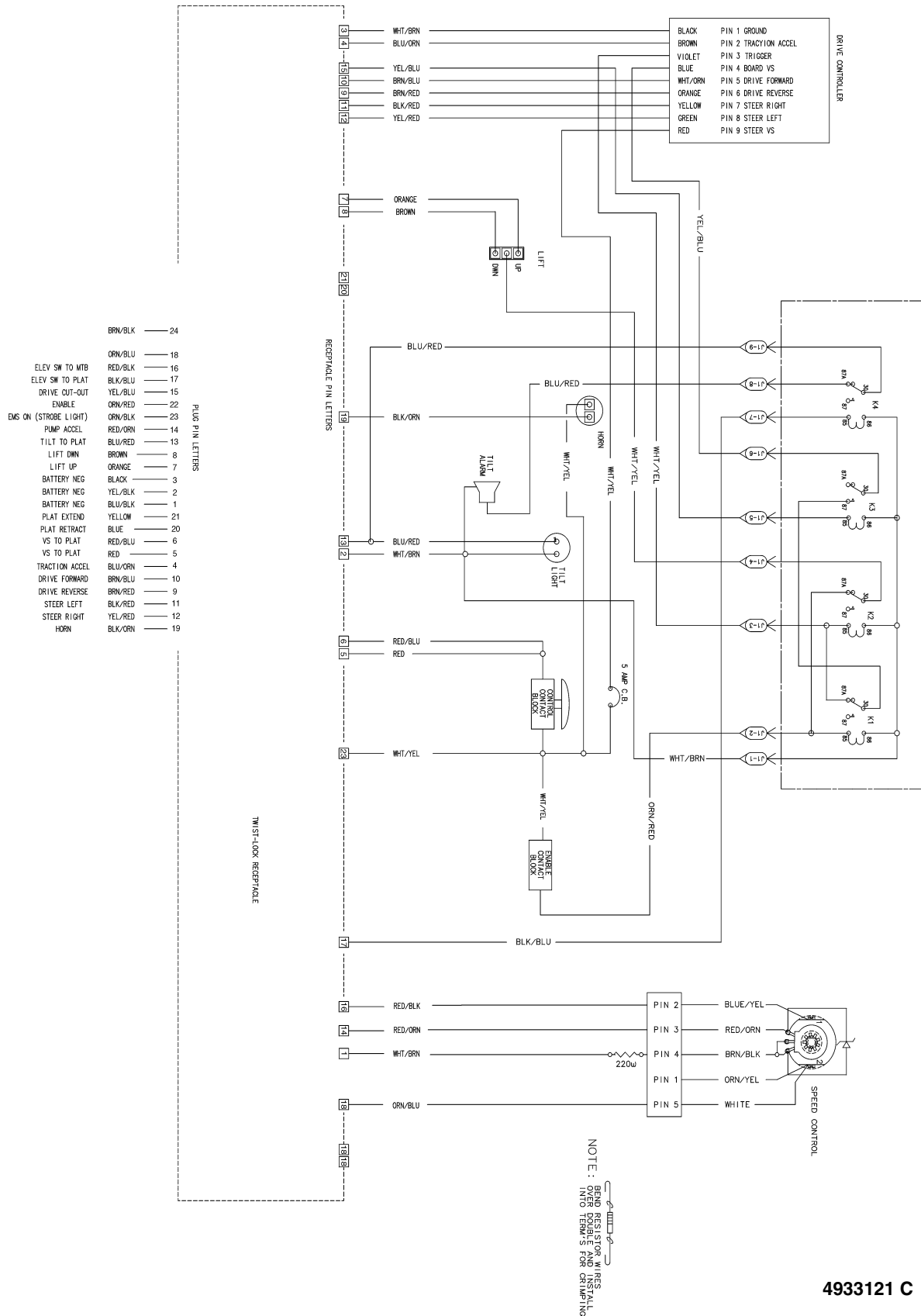
FIGURE 7-3.ELECTRICAL SCHEMATIC - PLATFORM (S/N 71506 TO PRESENT)
